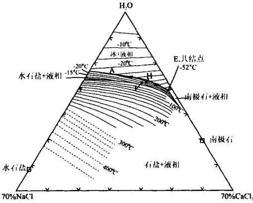
图 1 流体包裹体 CaCl 2 -NaCl-H 2 O 体系相图 [10] Fig. 1 Phase diagram of CaCl 2 -NaCl-H 2 O system in fluid inclusion
